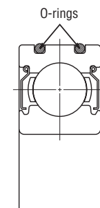
Fig. 1 Structure of Creep-Free Bearings
