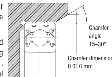
Fig. 5 Housing Shape and Dimension
